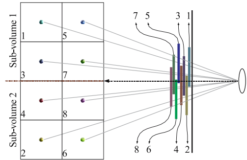
Fig. 6. Interleaving between subvolumes and selecting a suitable axis permutation remedies the PBTF problems in this example
