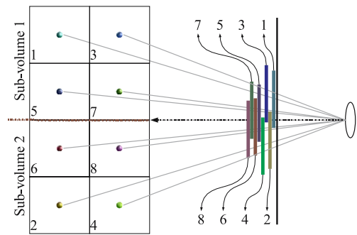
Fig. 5. Subvolume interleaving by itself is not sufficient to remedy the PBTF visibility problems. In this simple case, in spite of interleaving, voxels 3 and 4 have been incorrectly composited before voxels 5 and 6
